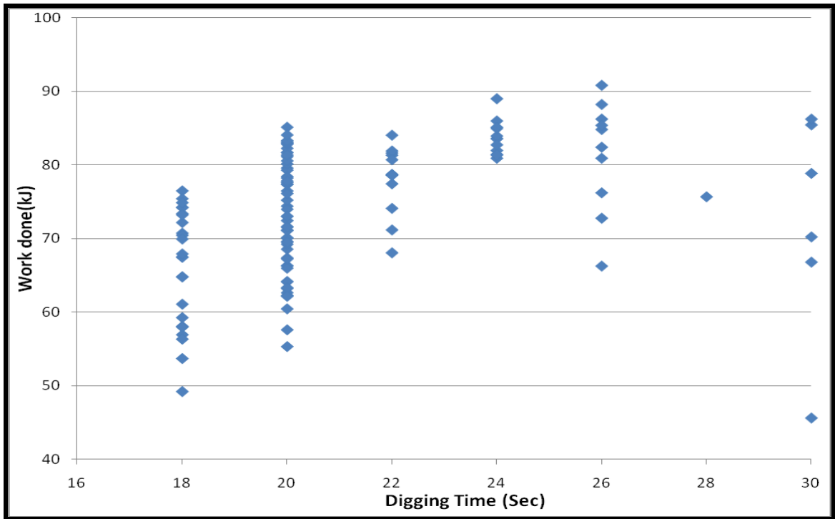
Figure 5.1 Work done (kJ) against the digging time (sec)
